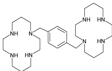
Figure 1: Structural Formula
